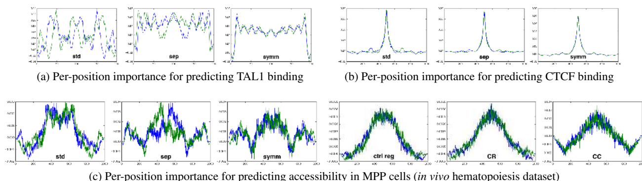
Figure 4: SFC layers improve per-position importance scores. Importance scores were computed on the input sequences using gradient \times input as described in Shrikumar et al. [2017a] for the best performing model over 10 random seeds. Scores at each position were averaged across multiple sequences and visualized. Blue lines represent the original per-position importance. Green lines are mirror images of the corresponding blue lines (they are included to aid with visually assessing symmetry). a: per-position scores for TAL1 task in simulated TF-binding, averaged over 100K generated sequences. b: per-position scores for in-vivo CTCF task, averaged over regions in the testing set. c: per-position scores for MPP accessibility task in hematopoiesis dataset, averaged over 10K regions.
