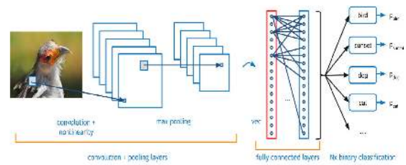
FIGURE 6. Convolutional neural network.
