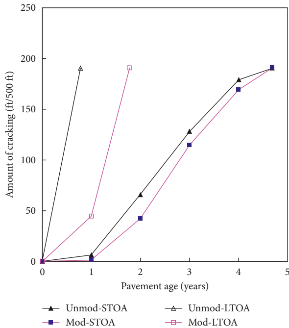
FIGURE 7: Effect of aging on thermal cracking of AOX-modified and unmodified asphalt mixtures (from Apeageyi [167]).
