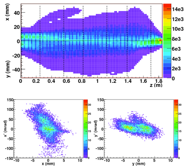
Figure 4: Trajectory plot (above) and output emittances ( \epsilon_{x,rms}=0.91\pi\text{mmrad} ; \epsilon_{y,rms}=0.66\pi\text{mmrad} ) in the transversal plane (below) based on LEBT simulations, using the input data from the first pepper pot device ( \epsilon_{x,rms}=0.85\pi\text{mmrad} ; \epsilon_{y,rms}=0.86\pi\text{mmrad} ). Dotted vertical lines show the drift and solenoid boundaries.
