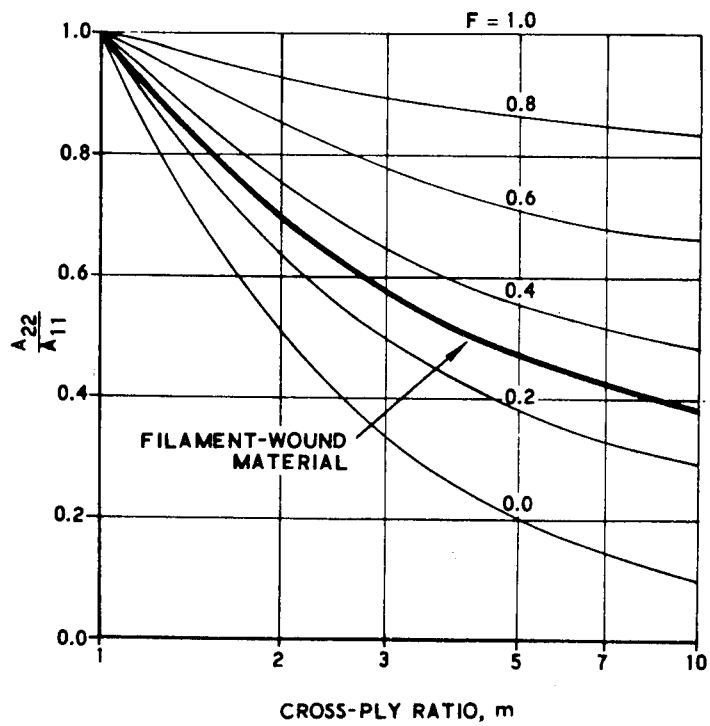
Figure 10. Dimensionless Stiffness Components A_{11} and A_{22}
