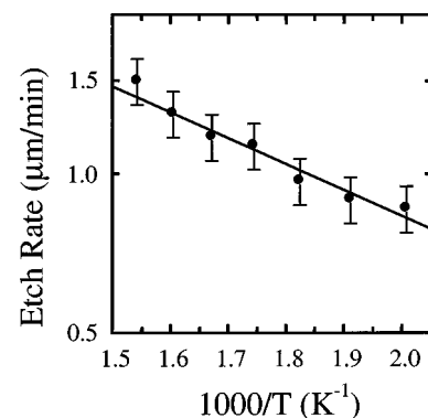
FIG. 6. Dependence of the etching rate on temperature between 225 and 375 °C. (The conditions were 300 W rf power, 15.5 Torr \text{CF}_4 , 11.4 Torr \text{O}_2 , 735 \pm 10 Torr He, and a nozzle-to-sample distance of 5 mm.)
