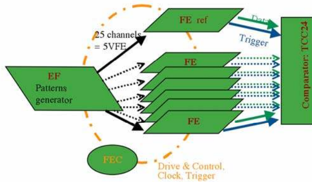
Figure 3: XFEST test bench
