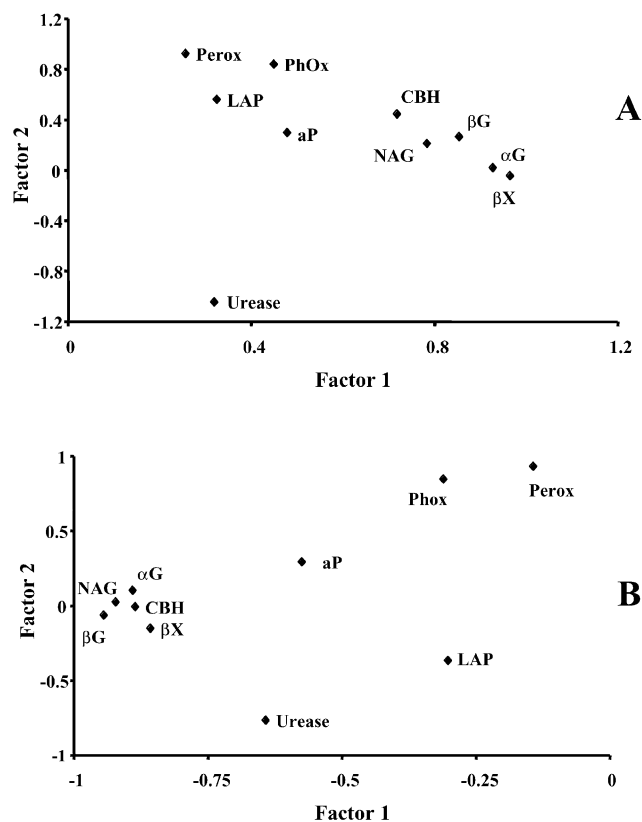
Fig. 2. Extracellular enzyme activity PCA factor loadings for soil control (A) and treatment (B) plots. For the control plots, factor 1 accounted for 43% of the variance, factor 2 accounted for 34%. In the treatment plots, factor 1 accounted for 50% of the variance, factor 2 accounted for 24%. Enzyme abbreviations are listed in Table 1.
