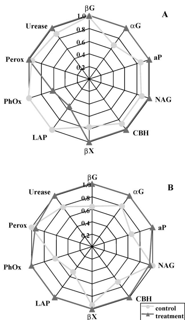
Fig. 1. Radar graphs illustrating the relative response of soil (A) and litter (B) extracellular enzyme activity to N deposition. Enzyme abbreviations are listed in Table 1.
