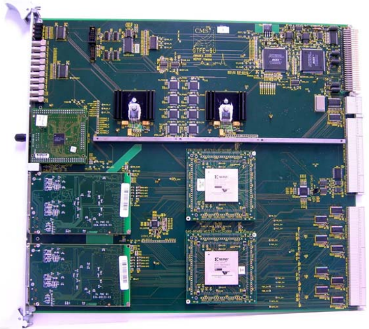
Figure 5 GTFE readout board
