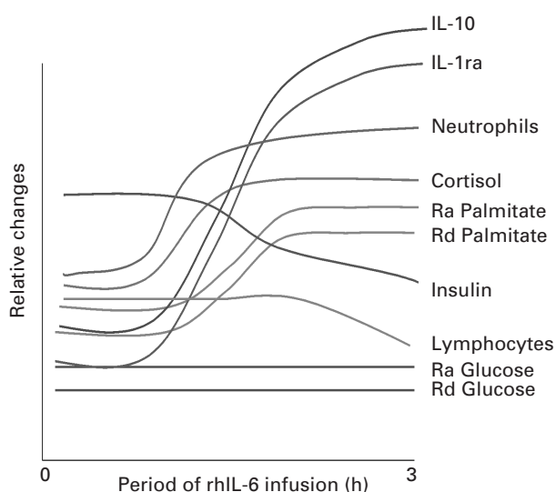
Fig. 1. Schematic representation of the cytokine response to exercise. The diagram illustrates the relative changes in a number of metabolic and immune variables in response to 3 h of infusion with recombinant human (rh) IL-6 eliciting plasma concentrations of IL-6 comparable with that obtained during exercise. The following variables are shown: rate of appearance (Ra) of glucose; rate of disappearance (Rd) of glucose; Ra of palmitate; Rd of palmitate; cortisol concentration, insulin concentration (reflecting data in patients with diabetes); the plasma concentrations of the anti-inflammatory cytokines IL-10 and IL-1 receptor antagonist (IL-1ra); numbers of circulating neutrophils and lymphocytes.
