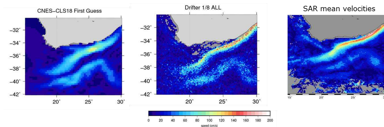
420 Figure 14: Mean velocities in the Agulhas Current area from (left) the GOCE-only derived MDT First Guess, (middle) drifting buoy velocities and (right) SAR derived mean velocities
