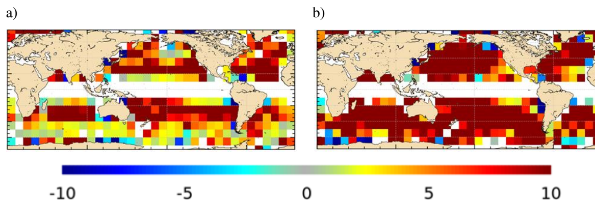
130 Figure 2: Difference (cm/s) of the RMSD obtained using the first guess of MDT CNES-CLS13 and the first guess of MDT CNES_CLS18 for the (a) zonal and (b) meridional components in 5°x5° boxes. Only boxes with more than 500 points and where difference is statistically significant at more than 95% (T-test) are shown. The reddish color underline improvement while bluish stand for degradation (see text for more detail)
