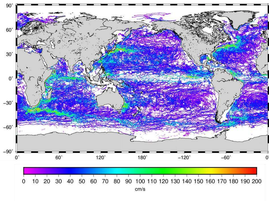
Figure 20: Trajectories of the 15m drogued SVP drifters available over year 2017. Colors give the speed velocities deduced along the drifter trajectories.
