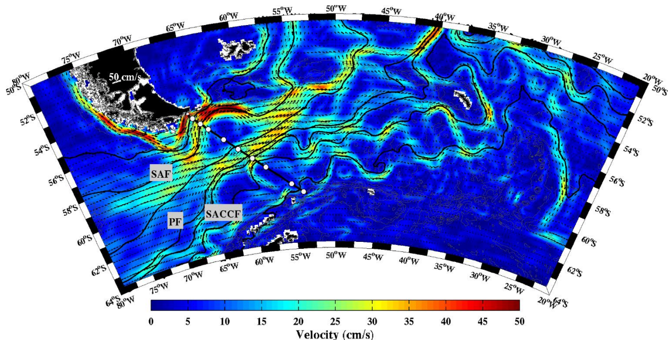
485 Figure 18: Mean surface velocity magnitude (in cm/s) and mean surface velocity vectors from MDT CNES-CLS18. Black lines are isolines of mean sea surface height corresponding to the main Antarctic Circumpolar Current (ACC) fronts and their branches: SAF-N (23 cm), SAF-M ( 0 cm), PF-N (43 cm), PF-M (-70 cm), PF-S (-79 cm), SACCF-N (-93 cm) and SACCF-S (-114cm). White dots indicate the position of the DRAKE moorings.
