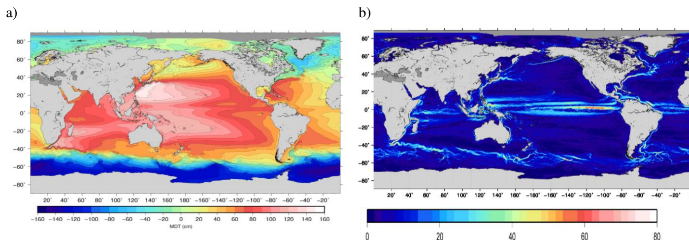
Figure 6: (a) The CNES-CLS18 Mean Dynamic Topography (cm) and (b) intensity of the associated mean geostrophic velocities
