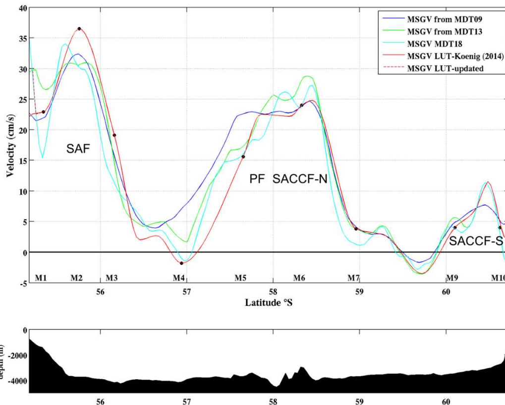
490 Figure 19: Mean surface geostrophic velocities (MSGV) derived from MDTCNES-CLS09 (blue), from MDTCNES-CLS13 (green), MDTCNES-CLS18 (cyan) and LUT (red) along Jason track #104. Location of the Drake moorings are indicated M1 to M10. Below bathymetry along the section.
