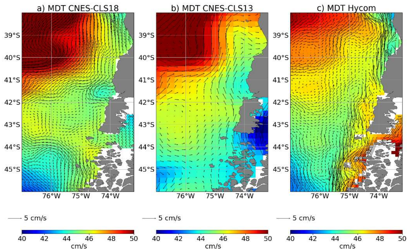
400 Figure 13: MDT and associated mean geostrophic current along the south Chilean coast from the MDT CNES-CLS13, MDT CNES-CLS18 and the numerical model HYCOM interpolated on the MDT CNES-CLS18 grid (1/8°)
