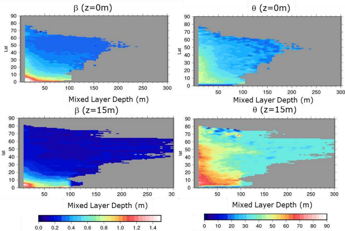
200 Figure 3: The \beta (left) and \theta (right) parameters calculated in this study as a function of Mixed Layer Depth and |latitude|. The top (resp. bottom) plots show the parameters at the surface (resp. 15m depth). Only bins with more than 50 values are shown.
