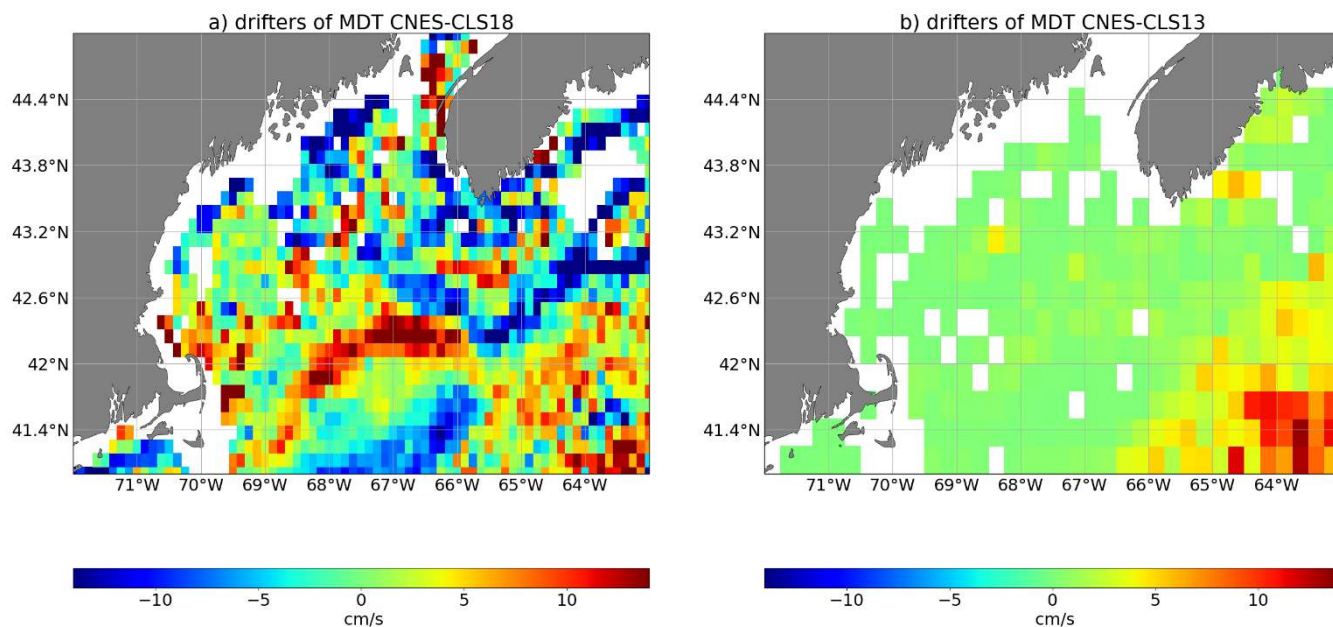
385 Figure 12: Zonal component of the mean synthetic velocities from drifters used in the computation of the (a) MDT CNES-CLS18 and (b) MDT CNES-CLS13
