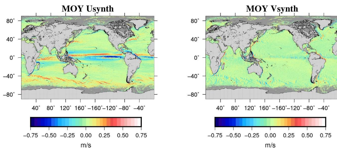
Figure 4: Mean zonal (left) and meridional (right) synthetic velocities
