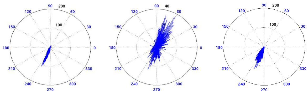
455 Figure 17: Ocean current roses of the (left) 30-day low-pass filtered ADCP observations, (middle) Copernicus-Globcurrent based on MDT CNES-CLS13 and (right) Copernicus-Globcurrent based on MDT CNES-CLS18. The numbers in blue indicate the angle of the ocean current direction (0° is eastward, 90° is northward). The numbers in black and the concentric circles give the number of occurrences in the observations for each angle. Note that for the middle plot, the scale is different regarding the occurrences.
