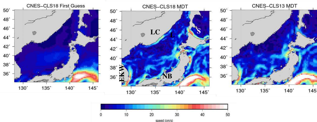
345 Figure 8: Mean geostrophic velocities in the Japan Sea in the CNES-CLS18 GOCE based First Guess (left), in the CNES-CLS18 MDT (middle) and in the CNES-CLS13 MDT (right). Abbreviations for the main currents are as follows: LC: Liman Current, EKWC: East Korean Warm Current, NB: Nearshore Branch of the Tsushima Warm current and SC: Soya current.
