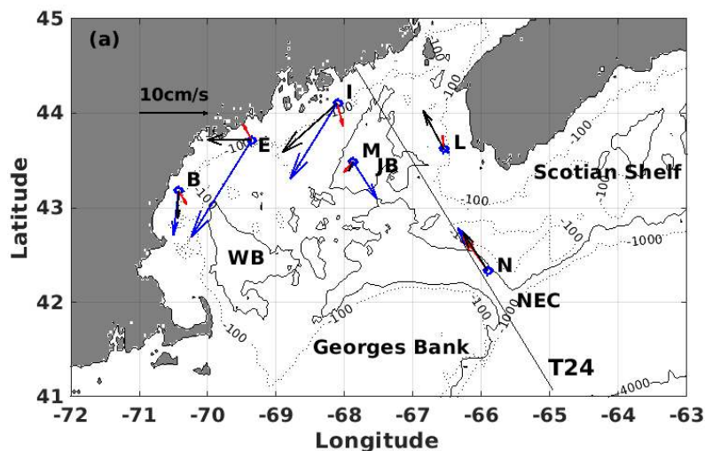
375 Figure 9: map of Gulf of Maine with the mean upper ocean (50m averaged) current vectors from in situ measurements at 6 buoy sites (N, L, M, I, E and B) in blue, and the mean geostrophic velocity vectors inferred from MDT_CNES_CLS13 in red and MDT_CNES_CLS18 in black. One Jason altimeter track 24 (T24) is also shown. (Abbreviations: JB: Jordan Basin; WB: Wilkinson Basin; NEC: Northeast Channel).
