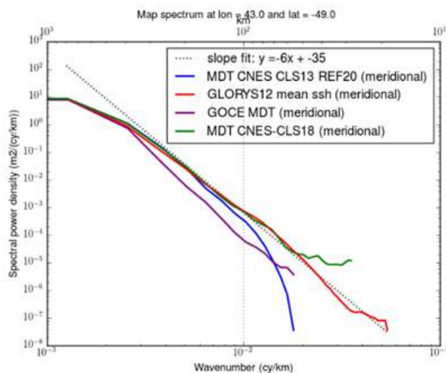
Figure 7: Spectral Power Density obtained for different MDT solutions
