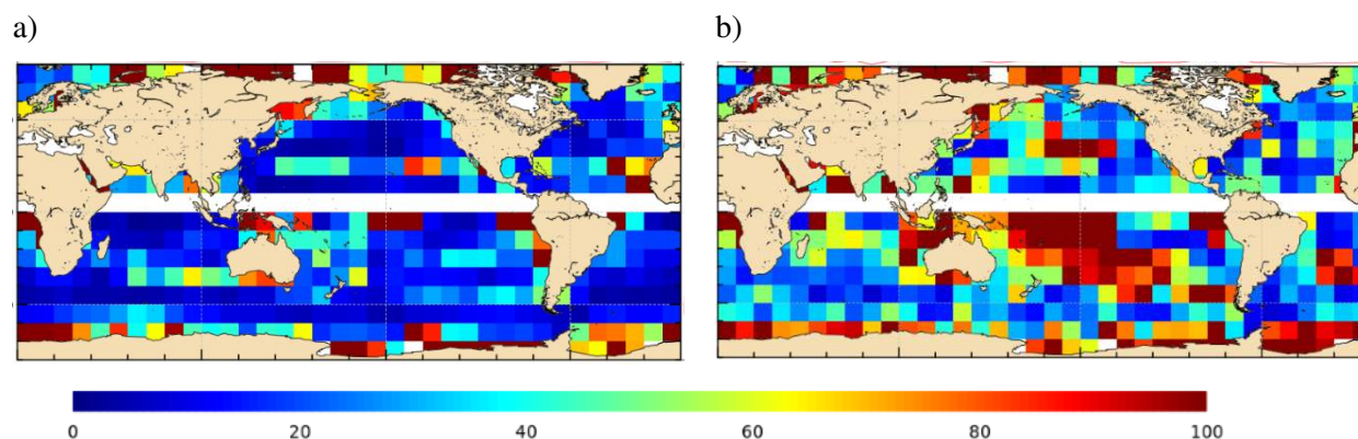
125 Figure 1: Root Mean Square differences between (a) zonal and (b) meridional mean geostrophic drifter velocities and the first guess geostrophic velocities in percentage of drifter variance (%) in 5°x5° boxes
