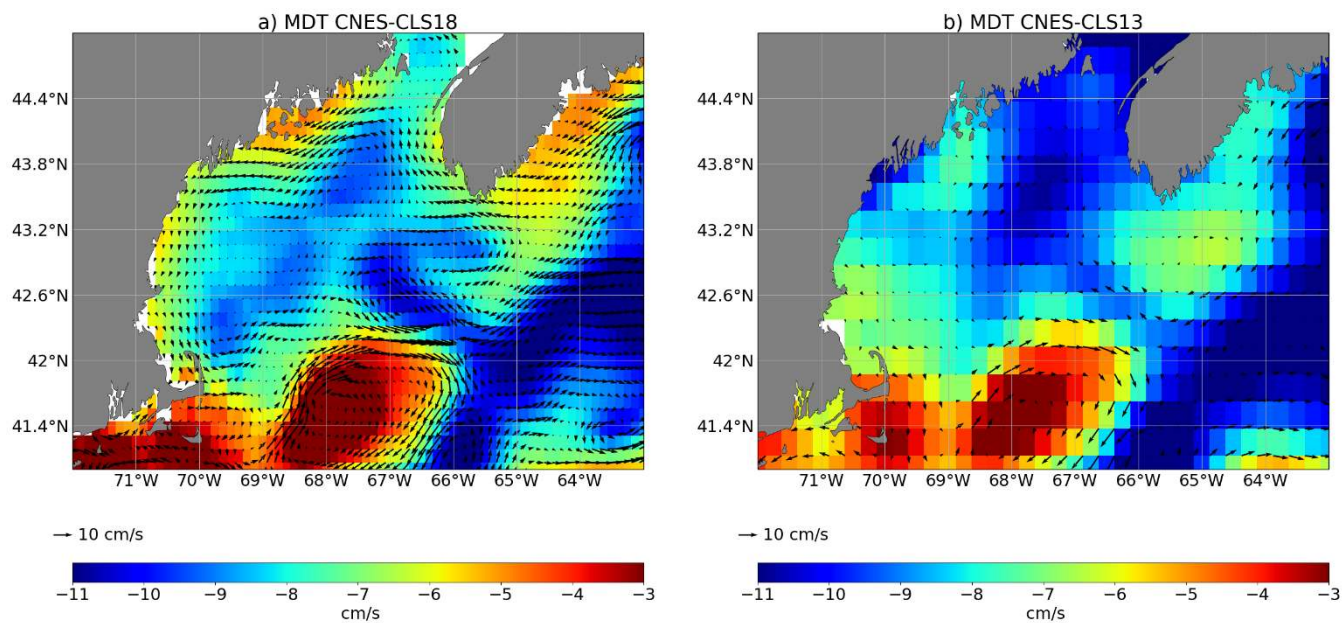
380 Figure 10: (a) MDT CNES-CLS18 and (b) MDT CNES-CLS 13 in the Gulf of Maine
