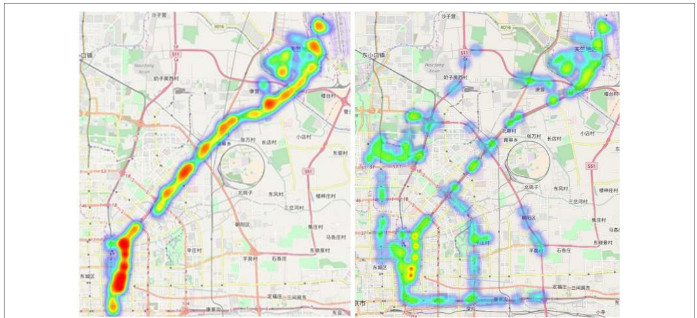
FIGURE 5 | Left: Unoptimized situation under consideration of cars causing traffic jam in the network. Right: Optimized redistributed cars using qbsolv. Note that the areas in red, which indicate high traffic density, are mostly absent from the right picture.
