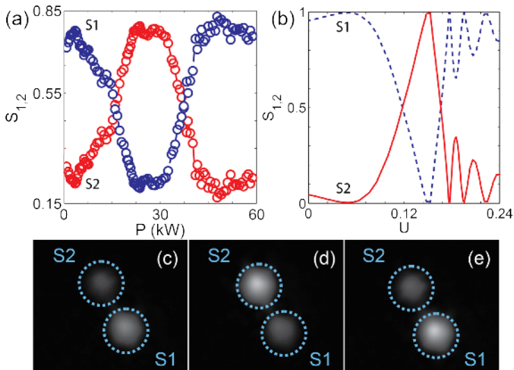
Fig. 2 (a) Experimentally measured power distribution between the two channels S1 (blue) and S2 (red) of the optofluidic coupler versus input power. (b) Theoretically calculated dependencies of power distribution on dimensionless input power U . (c)-(e) Measured intensity distributions at the output of the optofluidic coupler at (c) 3.5 \text{ kW} , (d) 24.2 \text{ kW} , and (e) 58.7 \text{ kW} .
