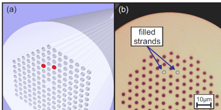
Fig. 1 (a) Illustration of an optofluidic coupler scaffolded by a photonic crystal fiber. (b) Microscope image of a fluid-filled photonic crystal fiber with two \text{CCl}_4 strands acting as nonlinear coupler.
