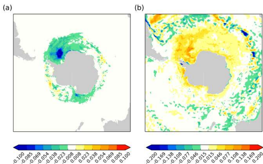
Figure 8. Impact of inclusion of active icebergs scheme instead of runoff-type input used in GO5: (a) difference in sea ice fraction, icebergs minus no icebergs; (b) difference in surface salinity (psu), icebergs minus no icebergs. In both cases means are taken over the second 5 years of a 10-year spin-up.
