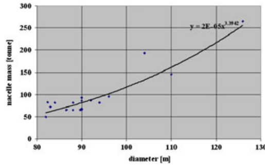
Figure 4. Mass as a function of size for nacelle considering only large size wind turbines.
