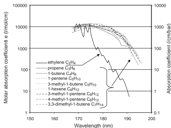
Fig. 5. The photon absorption coefficient for alkenes as function of wavelength. The decadic molar absorption coefficient, \epsilon , is defined by A = -\log_{10} T = \epsilon \times b \times c , where b is the path length in cm and c is the molar concentration in mol/l. The right-hand axis gives the absorption coefficient in units of /cm/bar for c = 0.044 mol/l. Data replotted from Refs. [19,20].
