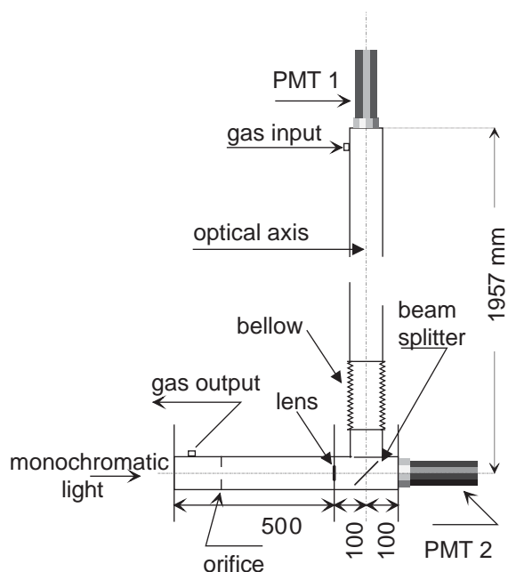
Fig. 2. Sketch of the working principle of the measuring system.
