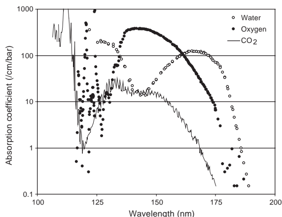
Fig. 3. The photon absorption coefficient for oxygen, water and carbon dioxide as function of wavelength. Data from Ref. [16].
