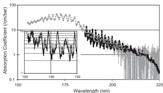
Fig. 7. The photon absorption coefficient as function of wavelength for C_2H_2 is shown for our data (+). The error bars corresponds to the total error. The solid line has been drawn according to data in Ref. [24]. The insert is a detailed view of the data between 185 and 195 nm.
