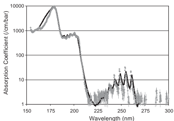
Fig. 6. The photon absorption coefficient as function of wavelength for C_6H_6 is shown for our data (+). The error bars corresponds to the total error. The solid line has been drawn according to data in Refs. [21–23].
