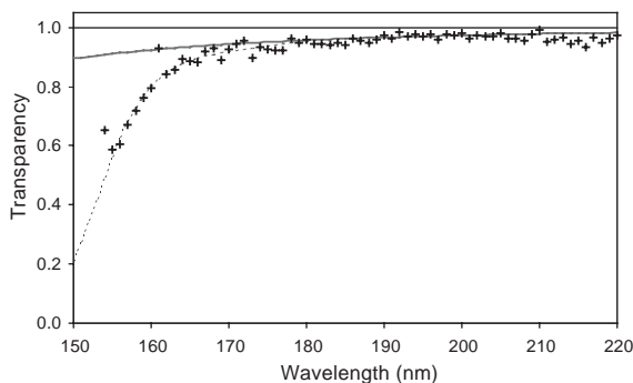
Fig. 13. Transparency as function of wavelength of C 4 F 10 for a photon path length of 186 cm at NTP (+). The solid line is Rayleigh scattering only. The dotted line shows the effect of adding 35 ppm of n-C 4 H 10 and the water and oxygen content which was measured to be 1 ppm.
