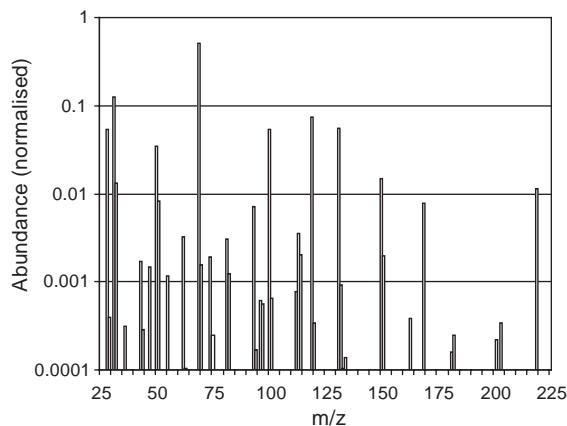
Fig. 8. Abundance of elements as function on m/z for a raw \text{C}_4\text{F}_{10} gas. The integral is set equal 1.
