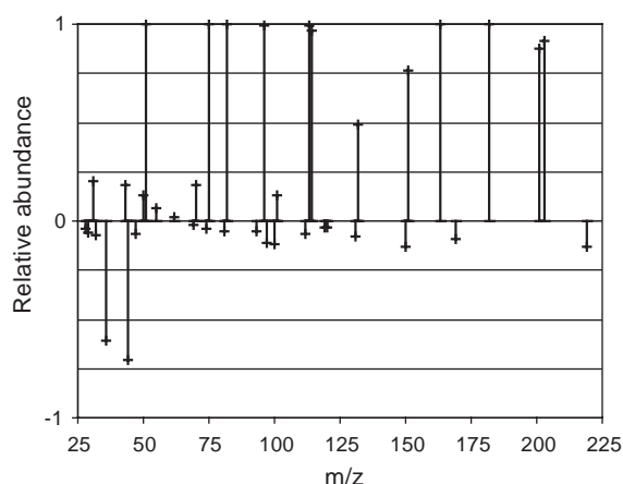
Fig. 9. Relative abundance of elements as function on m/z for a raw and a clean \text{C}_4\text{F}_{10} gas defined by the ratio (\text{Abundance}_{\text{raw}} - \text{Abundance}_{\text{clean}})/(\text{Abundance}_{\text{raw}} + \text{Abundance}_{\text{clean}}) .
