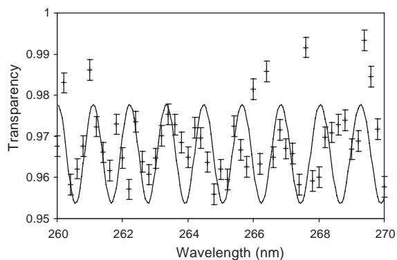
Fig. 11. The photon absorption in argon which had been flowed through activated carbon at 90^\circ\text{C} . The carbon had been saturated by raw C_4F_{10} . The error bars corresponds to the total error. The solid line is a fit with a period of 160\text{ cm}^{-1} .
