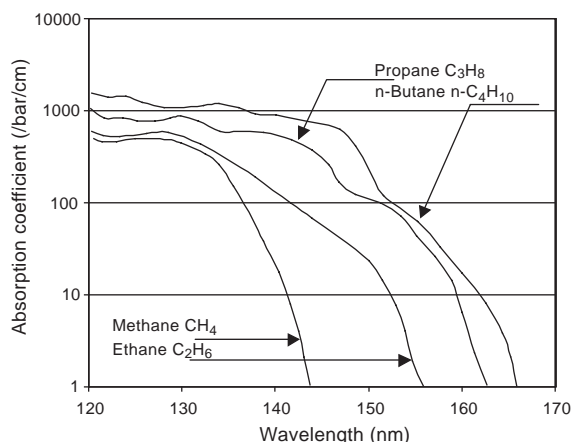
Fig. 4. The photon absorption coefficient for alkanes as function of wavelength at atmospheric pressure and 25°C. Data replotted from Refs. [19,20].
