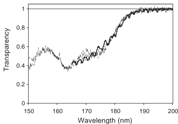
Fig. 10. Transparency as function of wavelength for sample [c] of C_4F_{10} for a 20 cm long photon path length at 2.3 bar absolute. The data points have been provided by the HADES experiment at GSI. The solid line is a possible fit with C_2H_2 at 130 ppm, C_2H_4 at 11 ppm, other alkenes at 0.3 ppm and C_6H_6 at 0.3 ppm.
