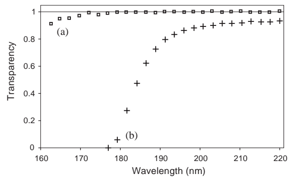
Fig. 1. Transparency as function of wavelength in two samples, [a] and [b], of \text{C}_4\text{F}_{10} for a 15 cm long photon path length at NTP. The oxygen and water contamination is, respectively, 4.3 and 5.0 ppm.
