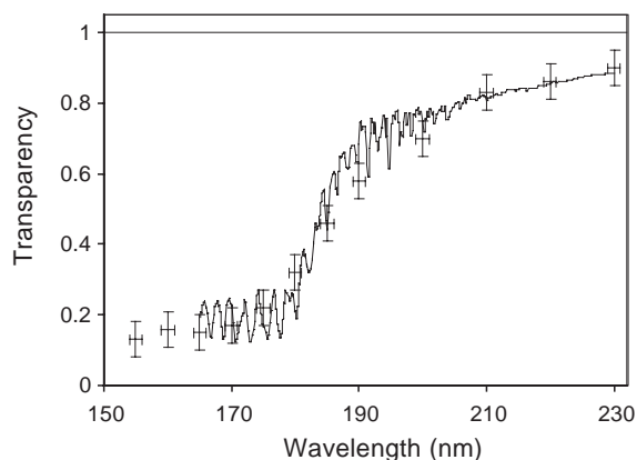
Fig. 12. Transparency as function of wavelength of a sample [d] of C_4F_{10} for a 500 cm long photon path length at NTP. The error bars corresponds to the total error. The solid line is a possible fit with C_2H_2 at 75 ppm, C_2H_4 at 0.025 ppm, other alkenes at 0 ppm and C_6H_6 at 0.05 ppm. Oxygen and water are set to the measured value of 2 ppm. Rayleigh scattering is also added for the 5 m scattering length.
