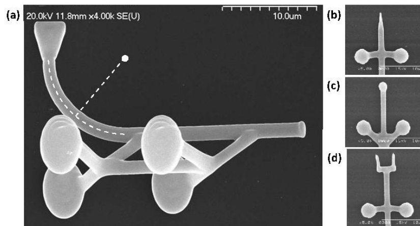
Fig. 2. SEM images of representative two-photon polymerized structures: a) A bent waveguide (bending radius R\sim 8 \mu\text{m} ; width \sim 1.5 \mu\text{m} ) sitting atop a supporting structure having spheroidal handles for optical trapping; the waveguide is connected via reverse-angled rods for minimal light-coupling loss the support structure; b) – d) Some tip structures that can be fabricated
