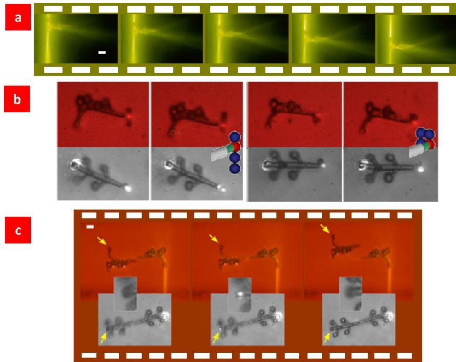
Fig. 5. Light coupling through a dynamically manipulated waveguide. (a) Snapshots from side-view fluorescent imaging of an optically trapped and manipulated waveguide (Media 4). (b) Snapshots showing selective fluorescence excitation of a target bead among a group of beads (left: vertical column of beads; right: 2×2 vertically arranged beads). (c) Snapshots showing reversed light coupling: an optically trapped structure creates a localized field and a second trapped structure is manipulated to scan the local field; the reverse-coupled light is visible from the top microscope (Media 5). The yellow arrow indicates where the light couples out when the scanning tip detects an optical field (scalebar:10 \mu m)
